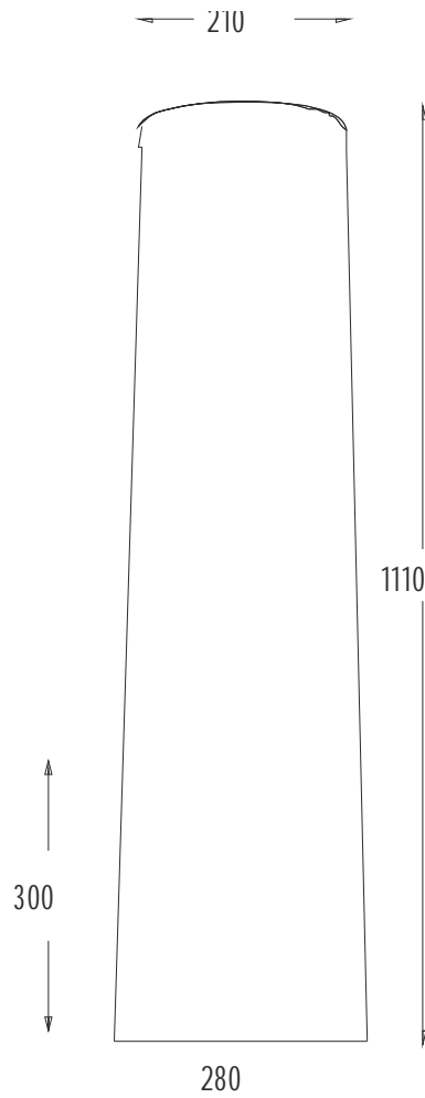
Modcon Bollards Type 001
